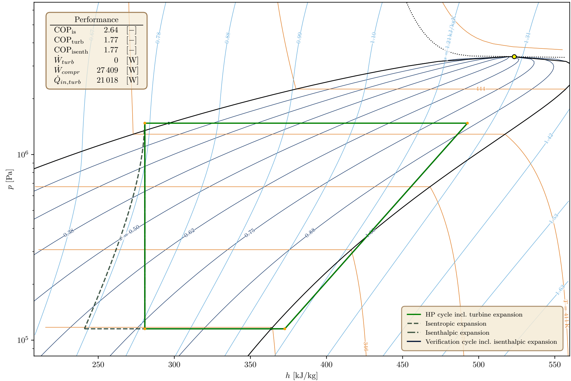
Conceptual Heat Pump Cycle – n – pentane
